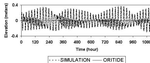
Figure 4. Model verification of sea surface elevation.
